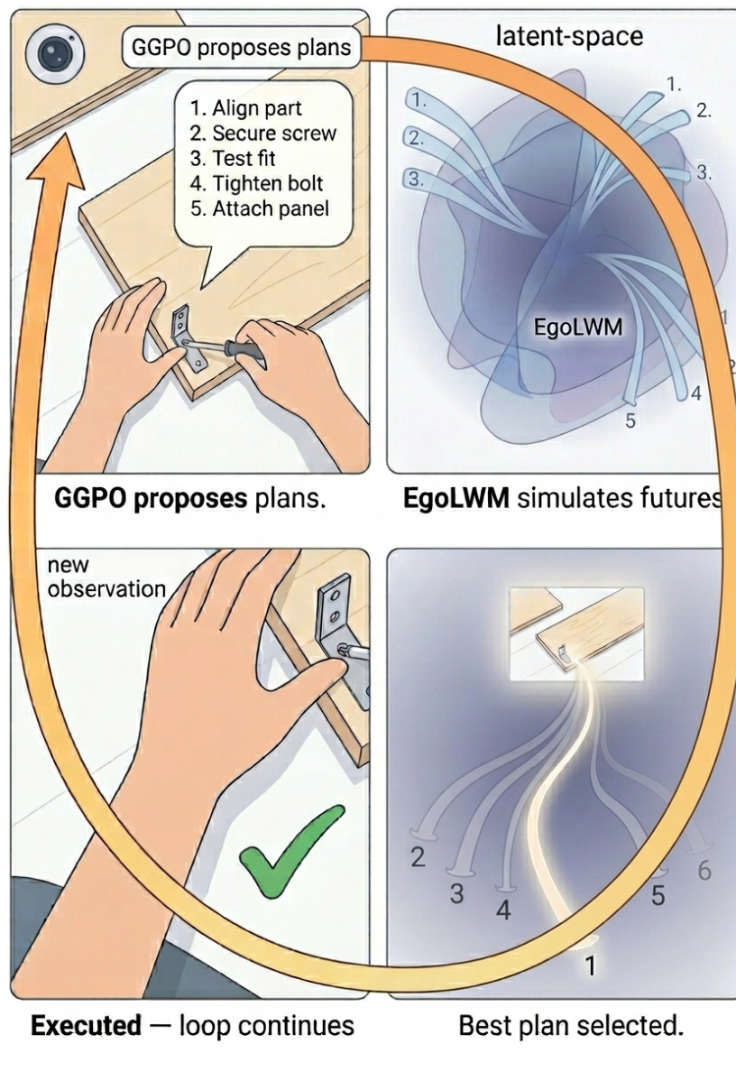
Figure 2: Integrated system architecture. GGPO generates K candidate step sequences, each serving as a language conditioning signal for EgoLWM. EgoLWM simulates the future semantic latent trajectories implied by each candidate and scores them against a goal latent. The highest-scoring plan is selected and executed; new egocentric observations feed back into GGPO, closing the loop. This tight coupling, where planning informs simulation and simulation informs planning, enables the system to anticipate failures before they occur rather than react to them after the fact.
