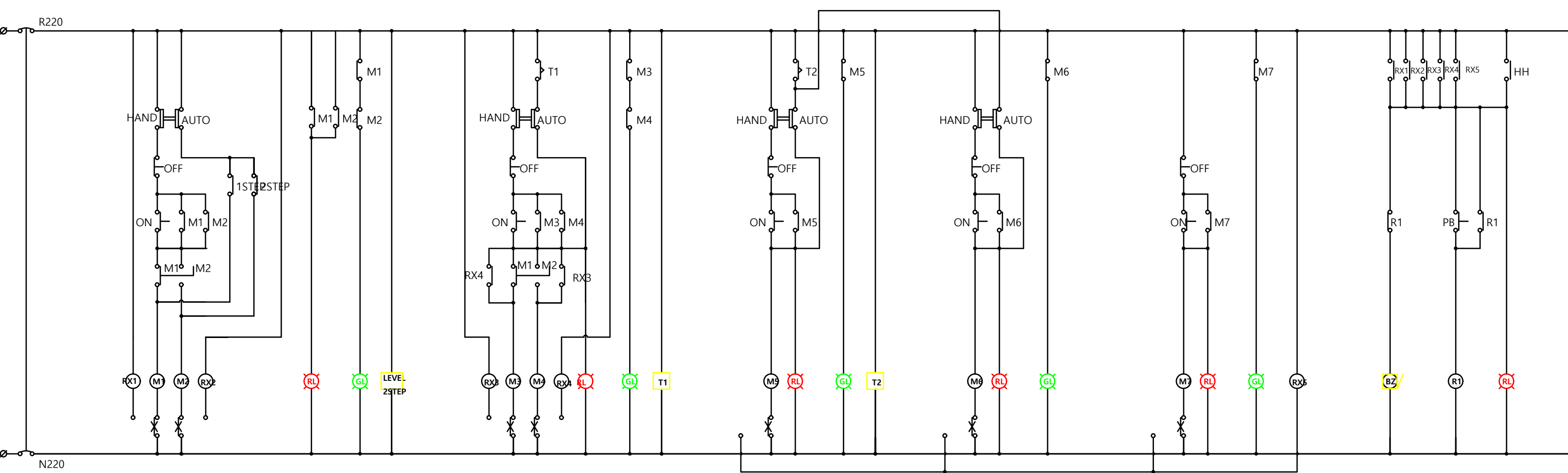
P-101A/B 배수펌프A/B ON,OFF,HAND/AUTO,M1/M2
