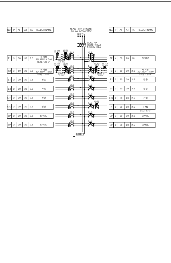
LE-B4-1 B4F 전기실 "A" TYPE
