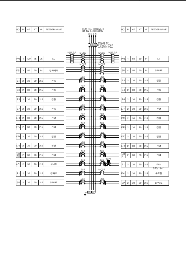
LE-B1 B1F EPS "A" TYPE
