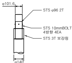
"B" DETAIL
