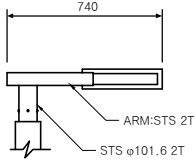
FIXTURE DETAIL
