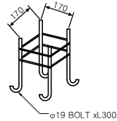
ANCHOR DETAIL
