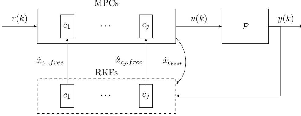
Figure 1: The dashed line emphasizes that each RKF operates independently from the others (apart from the shared initial estimate \hat{x} and the measured output y ), and therefore no computations are performed across filters. This independence does not hold for the MPCs: after each MPC solves its own optimization problem, an additional minimization problem is formulated that also incorporates past predictions, producing a single control input u along with an optimal tolerance and the corresponding best prediction \hat{x}_{best} .
