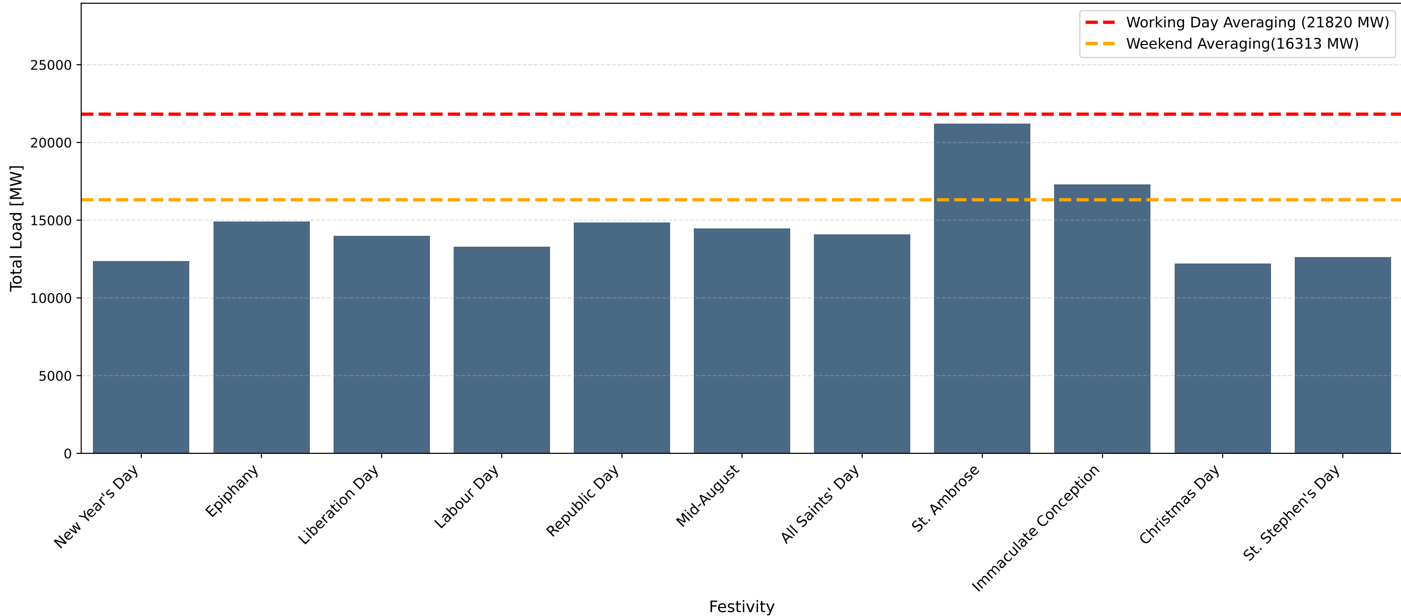
Averaging impact of the festivity on electricity demand (North Zone, 2021-2022)
