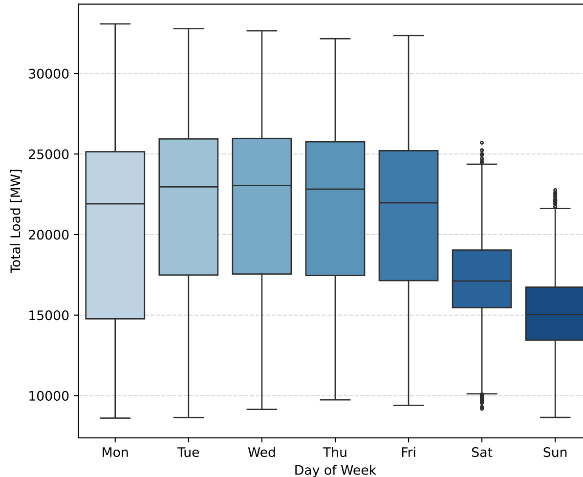
Weekly Seasonality: Load Distribution by Day of Week
