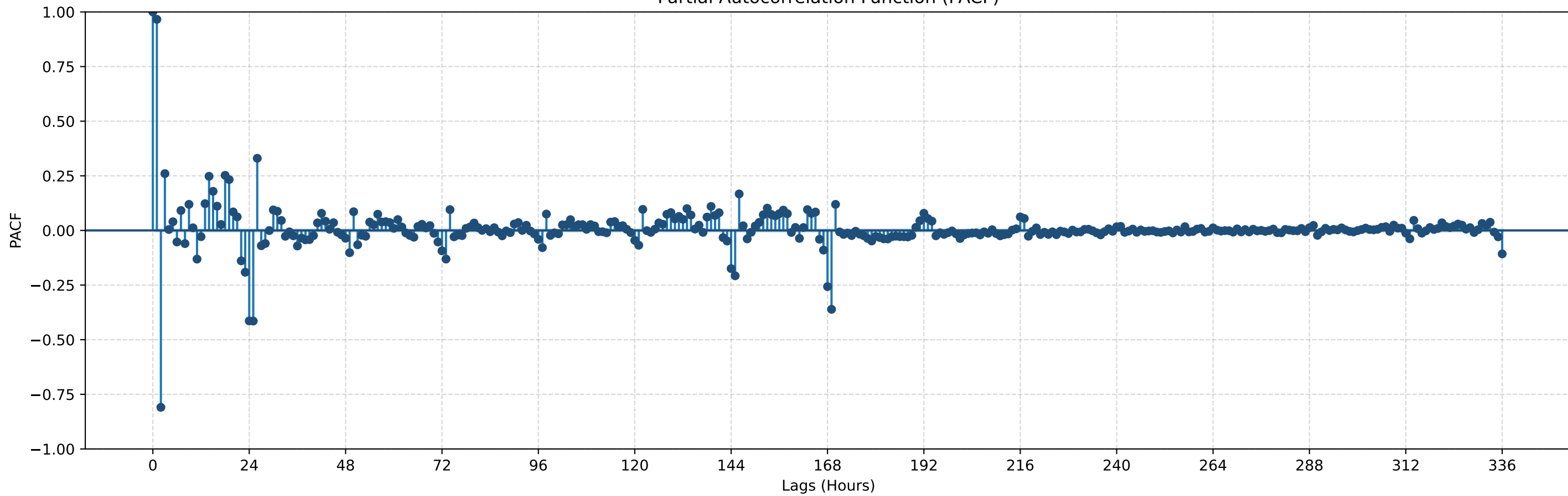
Partial Autocorrelation Function (PACF)
