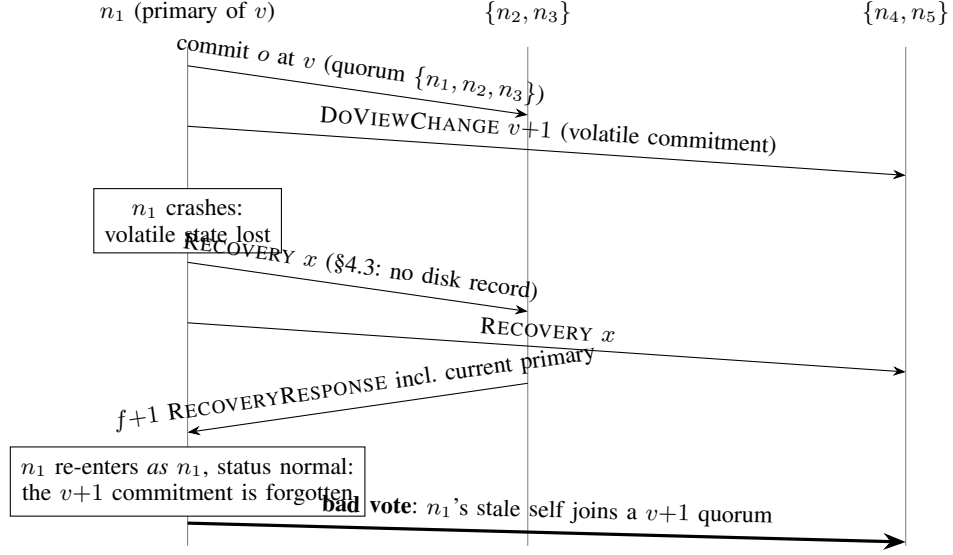
Fig. 2. The diskless-recovery amnesia of VRR at five voters ( f=2 ), after Michael et al. [4, Sec. 4.2 and Appendix A.1]. The forgotten commitment now spans a three-voter quorum: the recovering node's stale self can complete a v+1 quorum that a later leader cannot reconcile. Group arrows represent messages to each member; time runs downwards without a scale.
