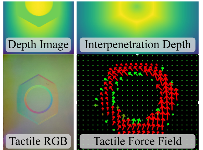
Fig. 12: Interpenetration rendered as a field. A compliant contact model turns the depth by which object and sensor overlap into the tactile image and the distributed force the policy reads; the overlap is the signal, not an artefact to be removed.
