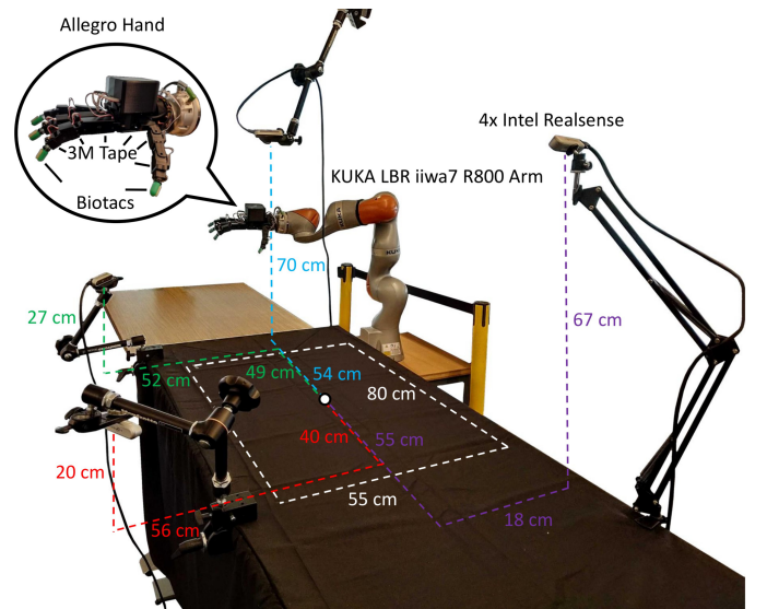
Fig. 15: A camera-based teleoperation cell, dimensioned. Four depth cameras around a marked table, a seven-axis arm and a four-fingered hand with tactile fingertips: the working volume in which every demonstration from this rig was recorded.
