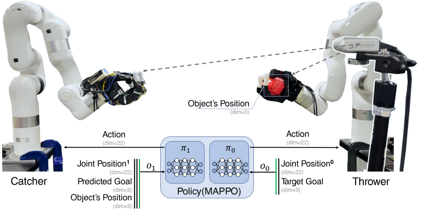
Fig. 25: Two arms and two four-fingered hands as thrower and catcher, with the observation and action dimensions each policy sees. The hands never touch: the coupling between them is the object’s flight.
