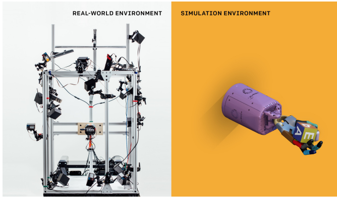
Fig. 28: The apparatus behind a headline in-hand reorientation number: a caged rig carrying sixteen motion-capture cameras and three RGB cameras, beside the simulated scene the policy was trained in. Reproducing the result means reproducing the left panel.
