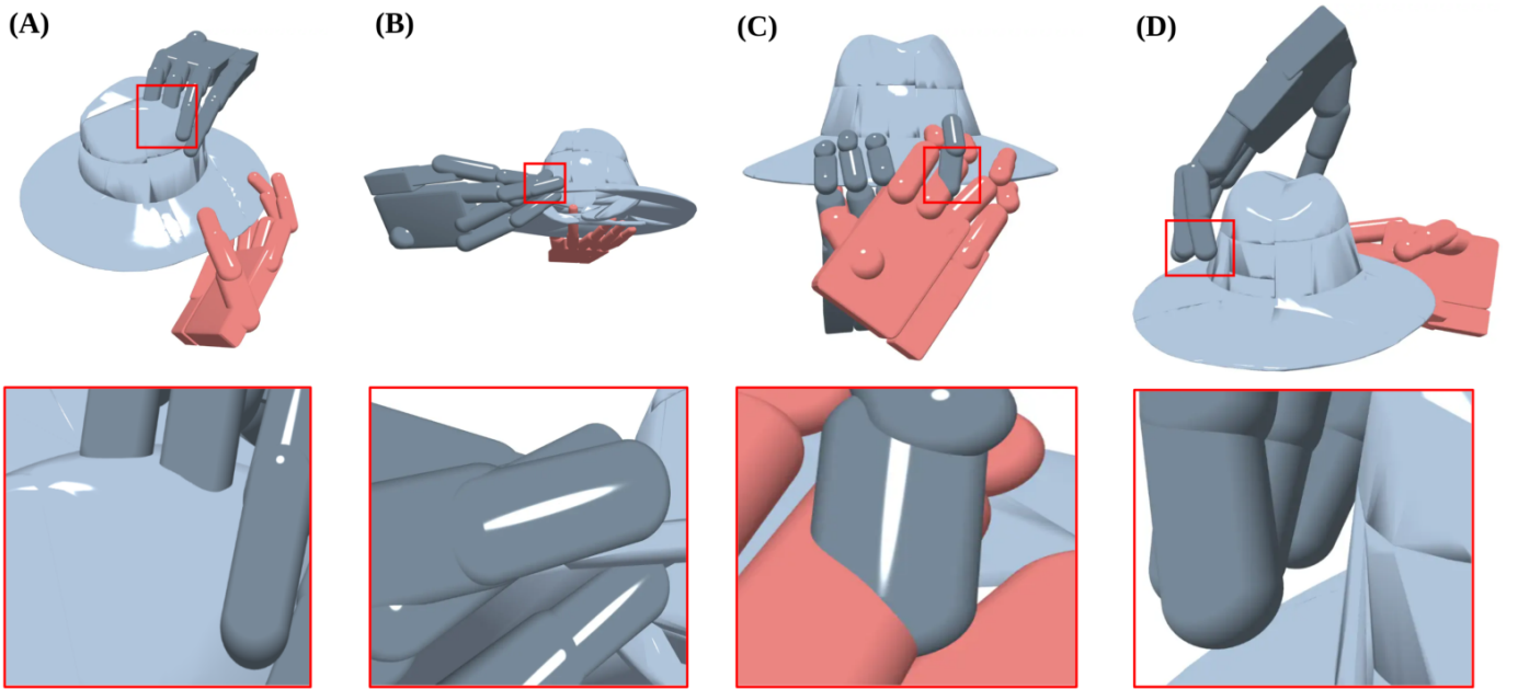
Fig. 23: The failure modes of synthesised two-hand grasps, with the contact region enlarged: fingers inside the object, fingers inside the other hand. At the scale of the whole grasp all four look plausible, which is why a success rate quoted without a penetration measure says little.
