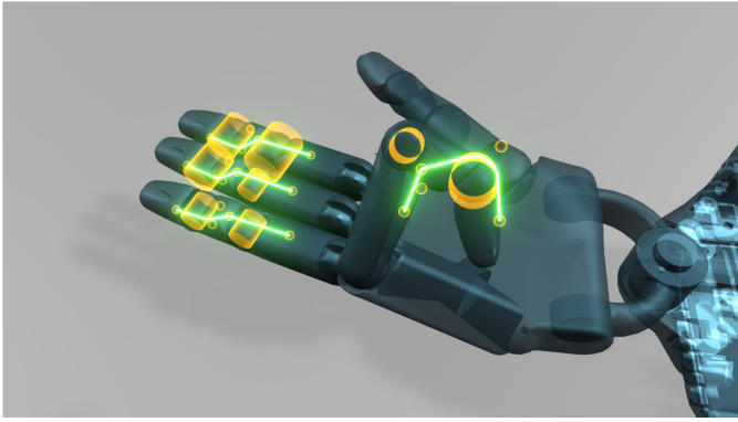
Fig. 13: A tendon-driven hand as the physics engine sees it: spatial tendons (green) routed over wrapping cylinders (yellow) inside the transparent shell. The routing geometry, not the joint limits, is what a sim-to-real gap on this hand is made of.
