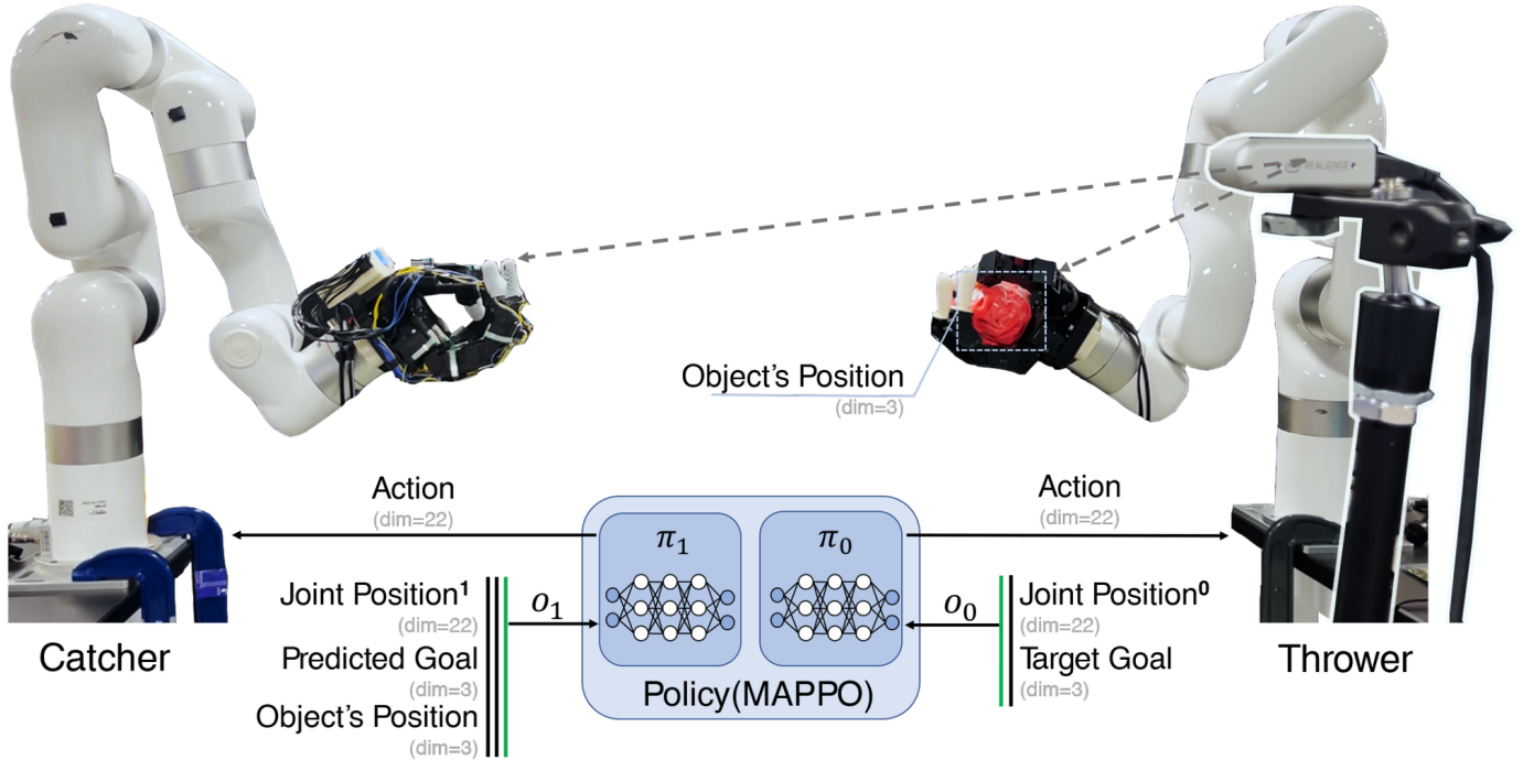
Fig. 21: Two arms and two four-fingered hands as thrower and catcher, with the observation and action dimensions each policy sees. The hands never touch: the coupling between them is the object’s flight.
