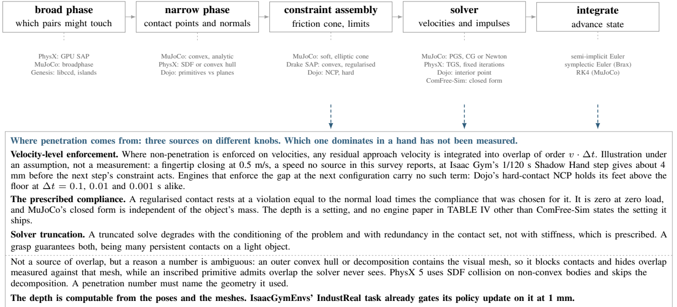
Fig. 10: One simulation step, and where engines differ. The stages every rigid-body engine runs, and under each the choices that separate the engines used for hands. The dashed arrows mark the three stages that make overlap: they do not answer to the same knob, and which of them dominates in a grasp is not measured anywhere in this corpus. The last note is not a source of overlap but a reason a penetration number is ambiguous.
