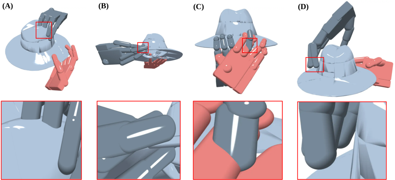
Fig. 24: The failure modes of synthesised two-hand grasps, with the contact region enlarged: fingers inside the object, fingers inside the other hand. At the scale of the whole grasp all four look plausible, which is why a success rate quoted without a penetration measure says little.
