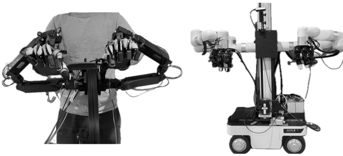
Fig. 17: The other end of the same problem: a worn bimanual exoskeleton that measures the operator’s own finger motion directly, and the mobile two-armed robot it drives. Greyscale; colour carried no information here.
