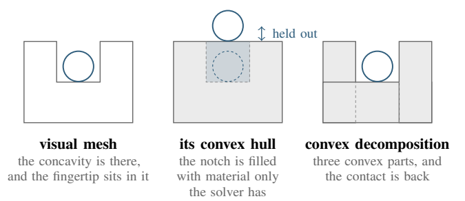
Fig. 4: The geometry the solver uses against the geometry the renderer draws. A single convex hull fills the concavity with material that exists only in the collision model, and holds the fingertip out of a contact the visual mesh allows.
