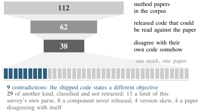
Fig. 9: Papers disagree with their own released code, and the funnel ends at the 9 the survey stands behind as contradictions. Section V-F classifies all 38 and names them.
