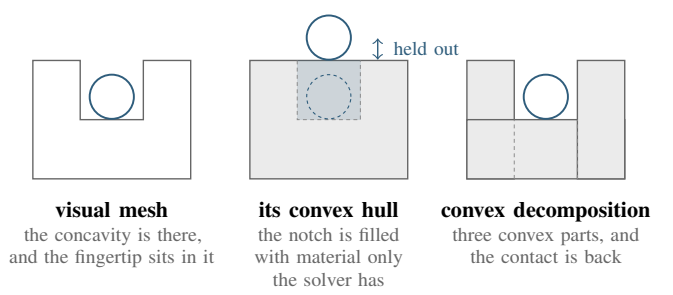
Fig. 5: The geometry the solver uses against the geometry the renderer draws. A single convex hull fills the concavity with material that exists only in the collision model, and holds the fingertip out of a contact the visual mesh allows.
