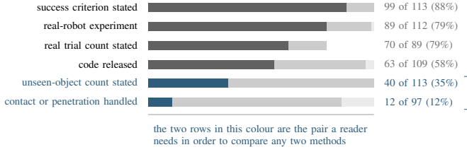
Fig. 13: What gets reported, and what does not. Each bar is a count of the 113 corpus method rows; the pale track behind it is the denominator that statistic is quoted against, printed beside the count, because four of the six are not 113. A faint tail past a track is the rows whose notes left that question unsettled. The two rarest reporting practices are marked in color.
