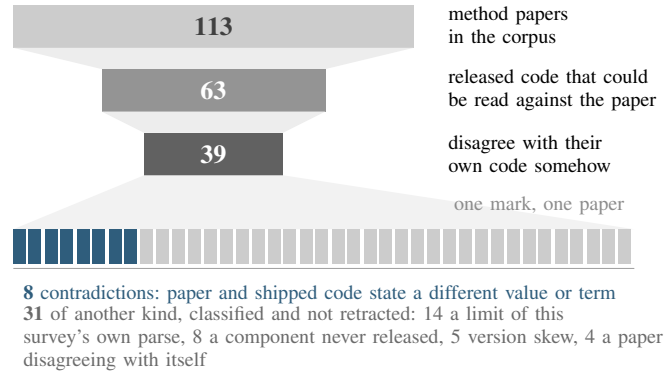
Fig. 9: Papers and their own released repositories state different things, and the funnel ends at the 8 the survey stands behind as contradictions. Table II names them, with the file and both values.
