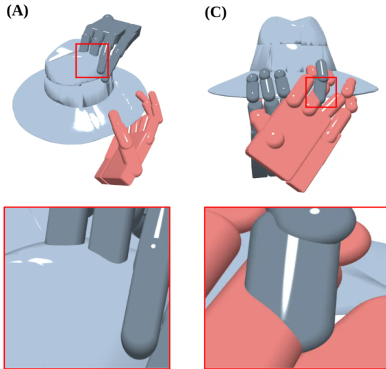
Fig. 12: Two failures of synthesised two-hand grasps, each enlarged at the contact: (A) a finger inside the object, (C) a finger inside the other hand. Both look plausible whole [41].
