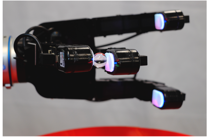
Fig. 8: Vision-based tactile sensors used as the fingertips themselves: each unit is a camera and an illuminated gel, and the sensor body sets the fingertip’s size and shape.
