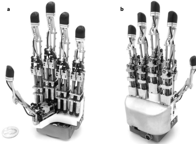
Fig. 4: A fully actuated linkage hand with the transmission left exposed: every joint is driven through its own metal four-bar and lead screw, with a coin for scale. Greyscale; the source photograph is near-monochrome [56]. The journal’s CC BY licence excludes anything marked there as third-party material; none is flagged on this figure, but the author should confirm.
