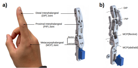
Fig. 5: Where the actuator count is cut: an anti-parallel linkage ties the distal joint to the proximal one, so one motor sweeps two joints and the finger’s reachable set is a curve rather than a surface. (Reproduced from [70].)
