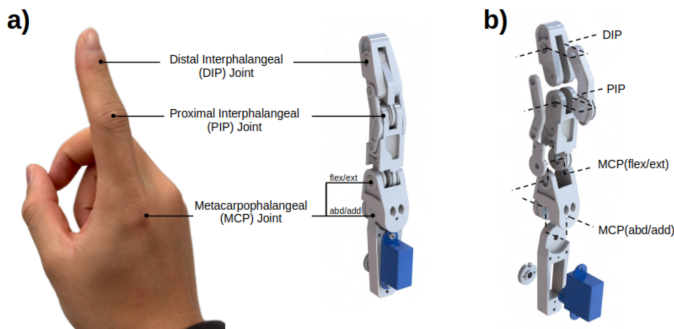
Fig. 4: Where the actuator count is cut: an anti-parallellogram linkage ties the distal joint to the proximal one, so one motor sweeps two joints and the finger's reachable set is a curve rather than a surface.
