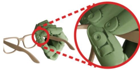
Fig. 9: What a retargeting error looks like at the contact. The pose on the left is plausible; magnified, the spectacle temple passes through the finger. Joint-angle error reports this as small. (Reproduced from [7].)
