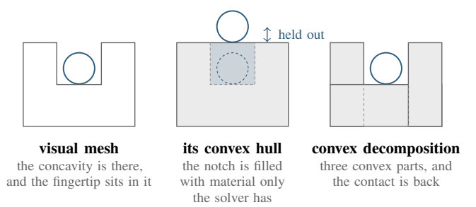
Fig. 5: The geometry the solver uses against the geometry the renderer draws. A single convex hull fills the concavity with material that exists only in the collision model, and holds the fingertip out of a contact the visual mesh allows.
