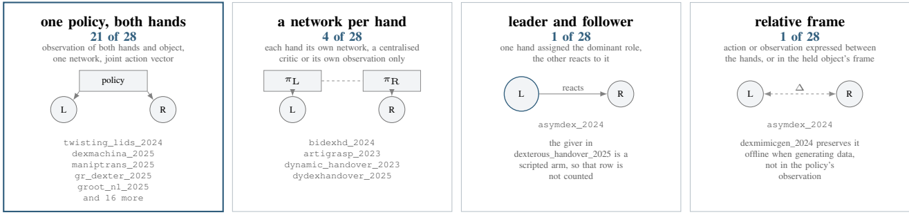
Fig. 11: Four ways to control two dexterous hands. Counts are over the 28 corpus rows that put a learned closed-loop controller on two multi-fingered hands, each read from its note. The four architectures do not partition the 28: AsymDex [59] is counted in both of the last two panels, being the only corpus paper that puts either mechanism inside a policy, and Bunny-VisionPro [61] and DexImit [165] are unassigned because their notes describe the rig and the data pipeline rather than the policy’s decomposition. The field is concentrated in the first panel; the two on the right are where the structure of the problem is actually used.
