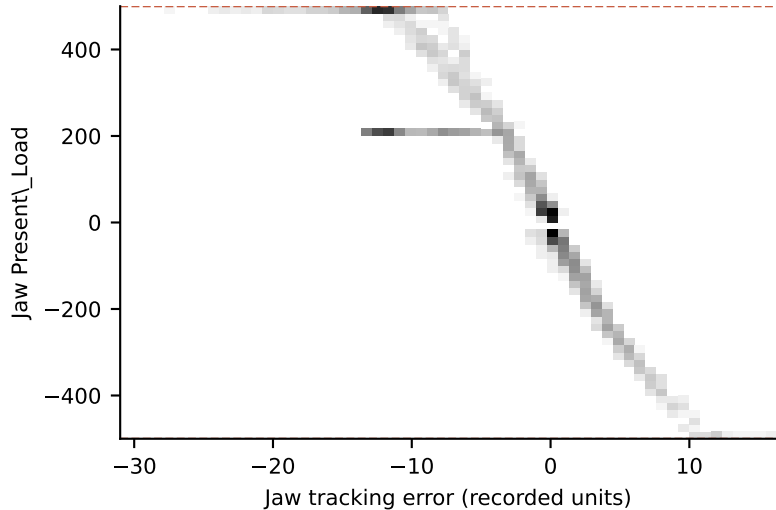
Teleoperation frames: 16.5% at the \pm 500 limit
