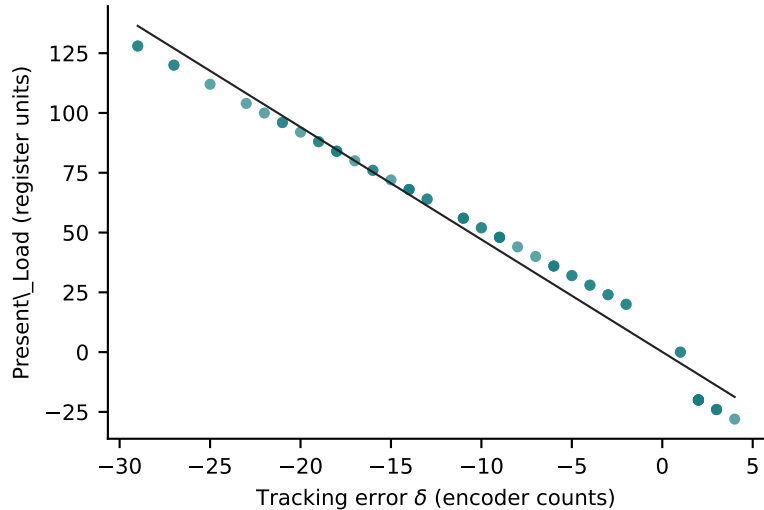
Static bench, one joint: 12 masses \times 5 poses, R^2 = 0.976
