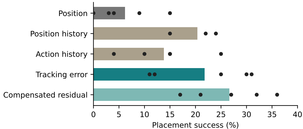
Simulation: mean and training seeds
