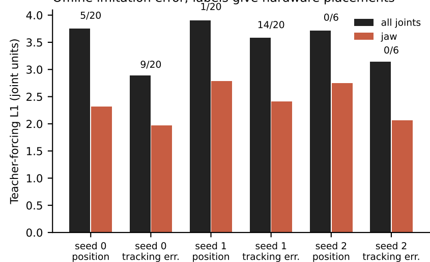
Offline imitation error; labels give hardware placements
