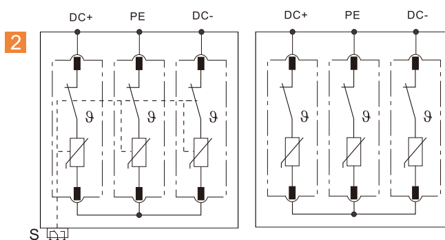
FXPV-12.5B/1000, FXPV-12.5B/1200, FXPV-12.5B/1500
