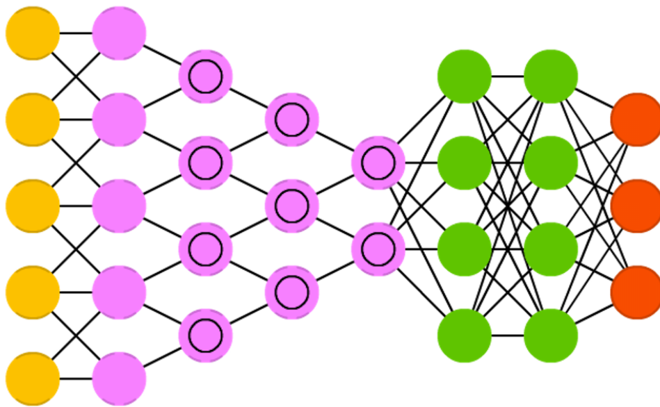
Figura 12 – CNN
