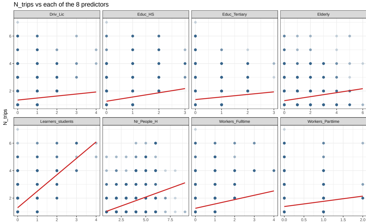
Figure 4: N_trips vs each of the 8 predictors (ggplot2)
