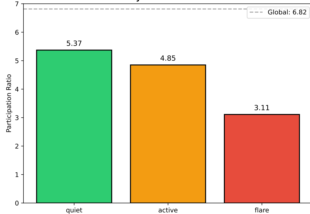
D Dynamical Constraint
