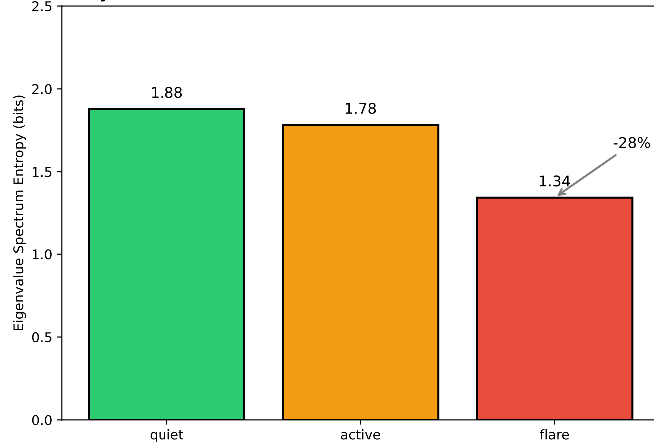
D Dynamical Constraint
