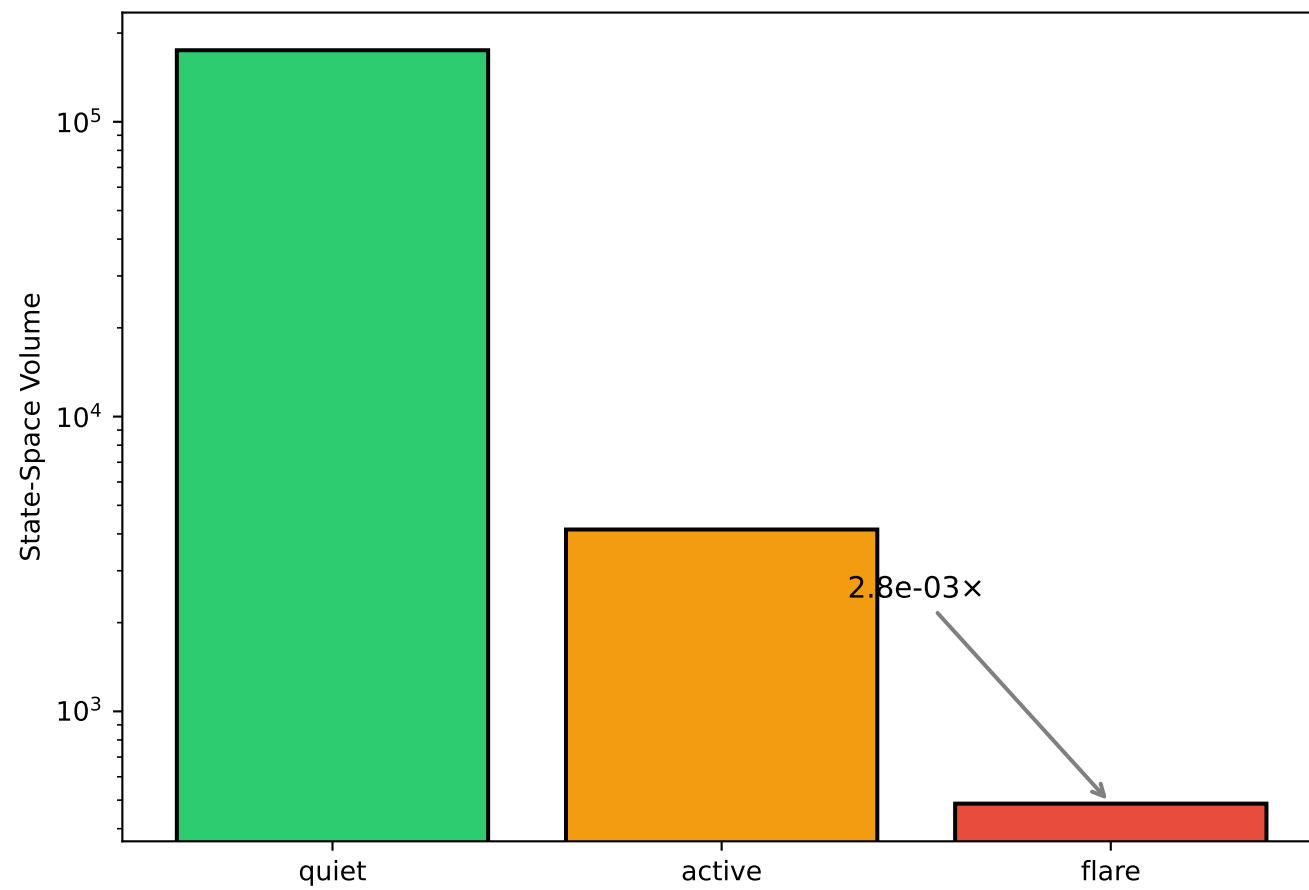
C Volume Contraction
