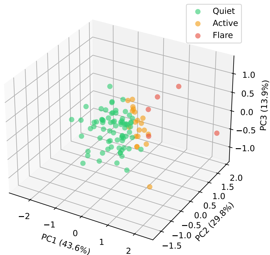
A State Space Projection
