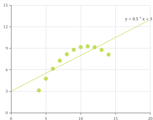
Anscombe's quartet
