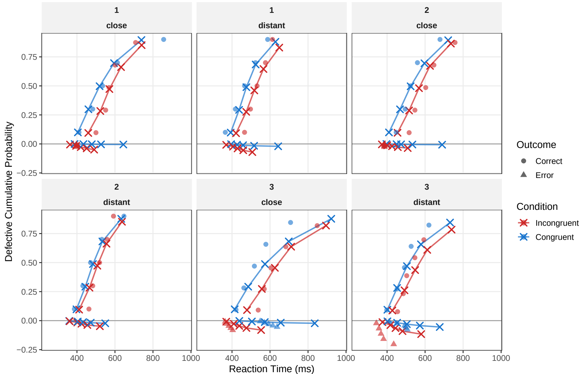
Quantile Probability Plot Corrects ( >0 ) \leftarrow 0 \rightarrow Errors ( <0 )
