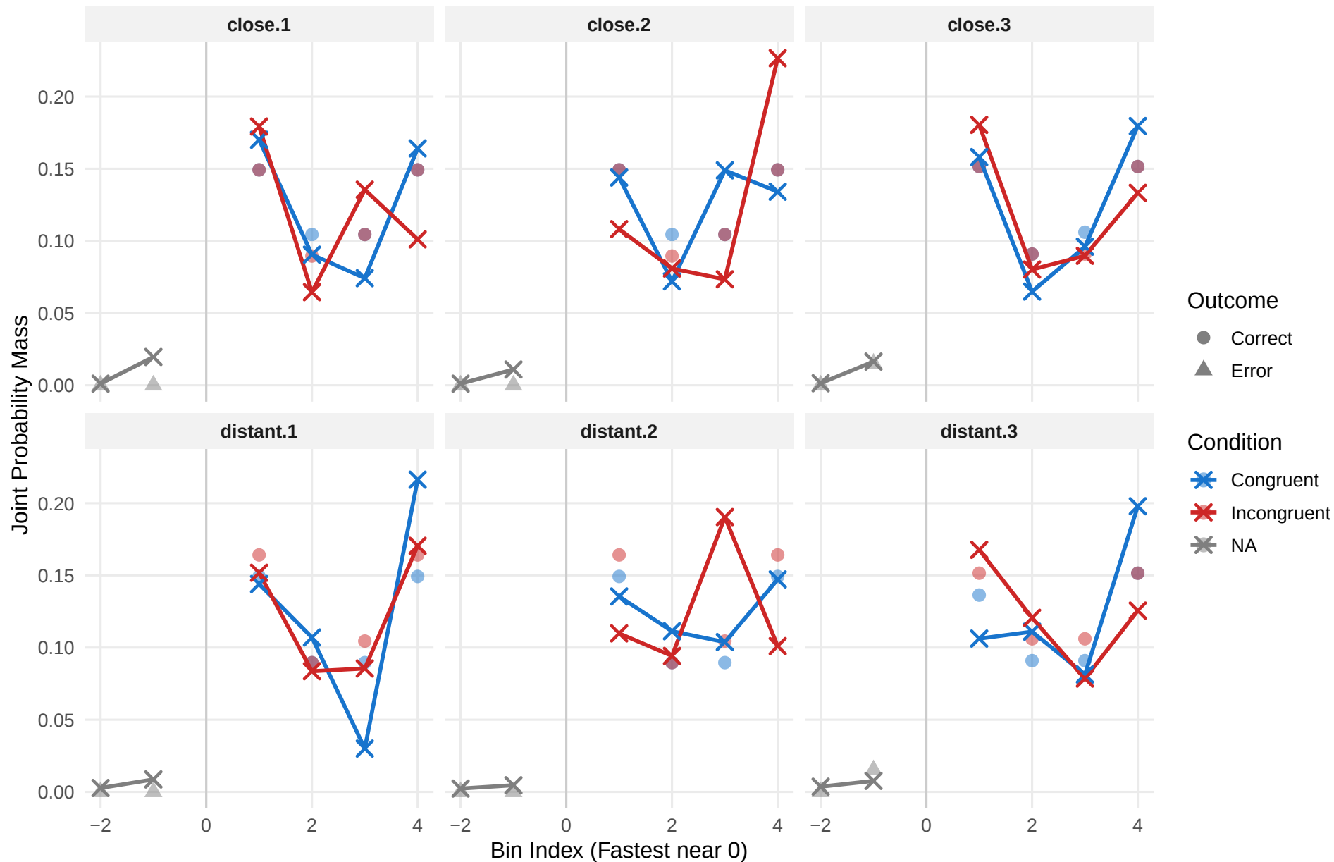
G-Square Fit: Probability Mass per Bin Errors (Left) <---- 0 ----> Corrects (Right) | Symbols = Obs, Crosses = Pred
