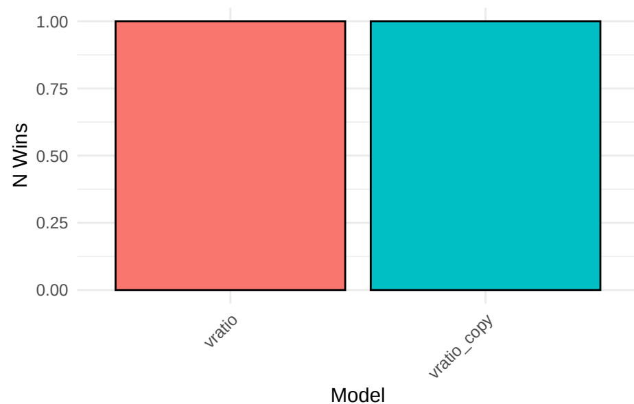
Subject Preferences
