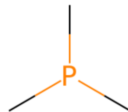
ligand6-0
