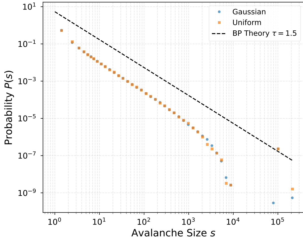
Avalanche Size Distribution
