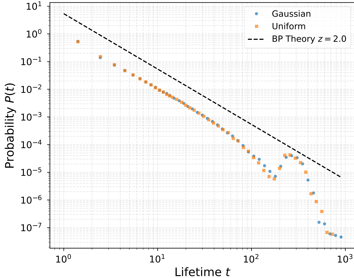
Avalanche Lifetime Distribution
