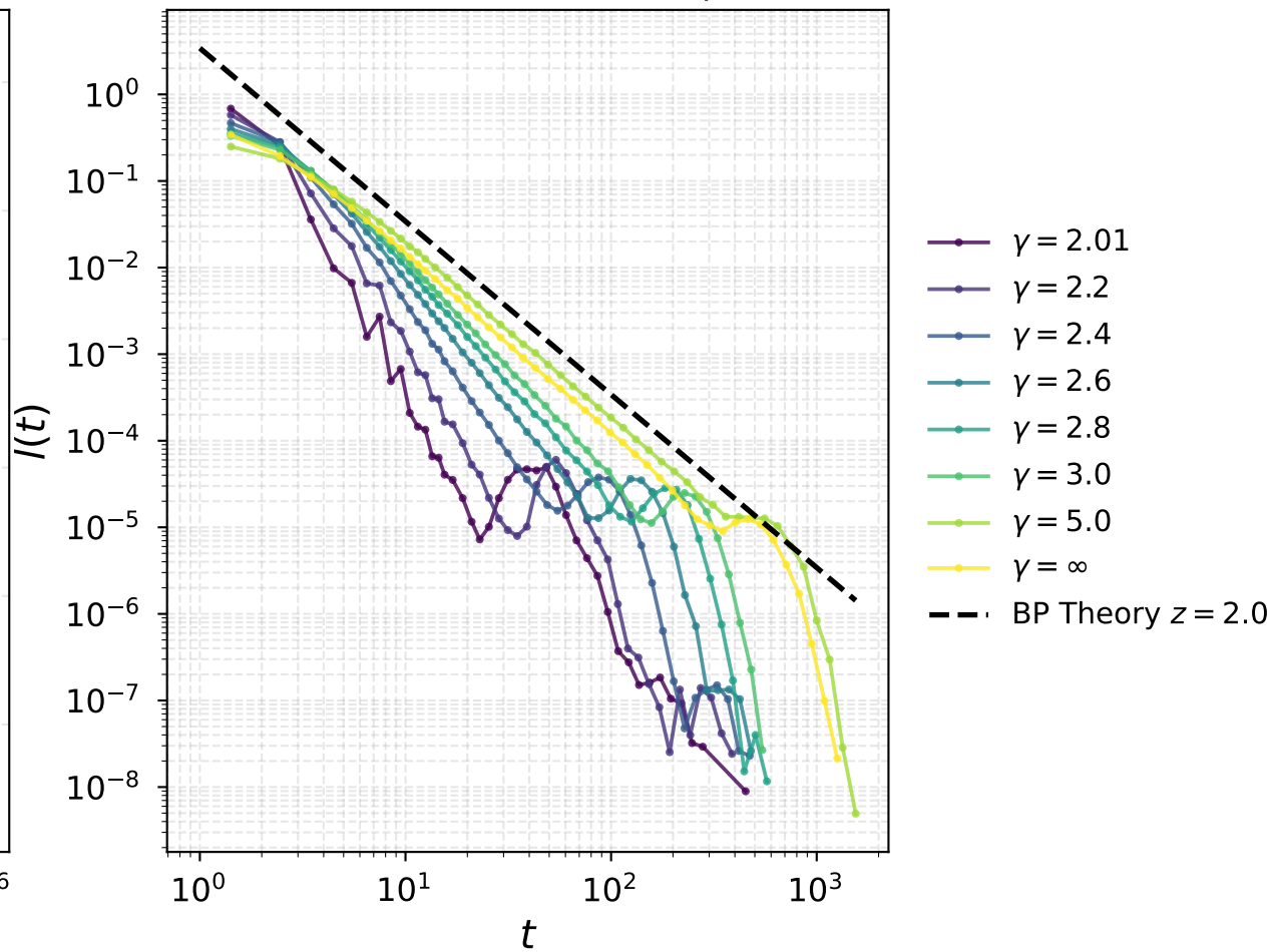
Avalanche Lifetime Distribution ( \gamma Scale-Free)
