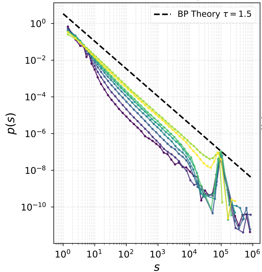
Avalanche Size Distribution ( \gamma Scale-Free)
