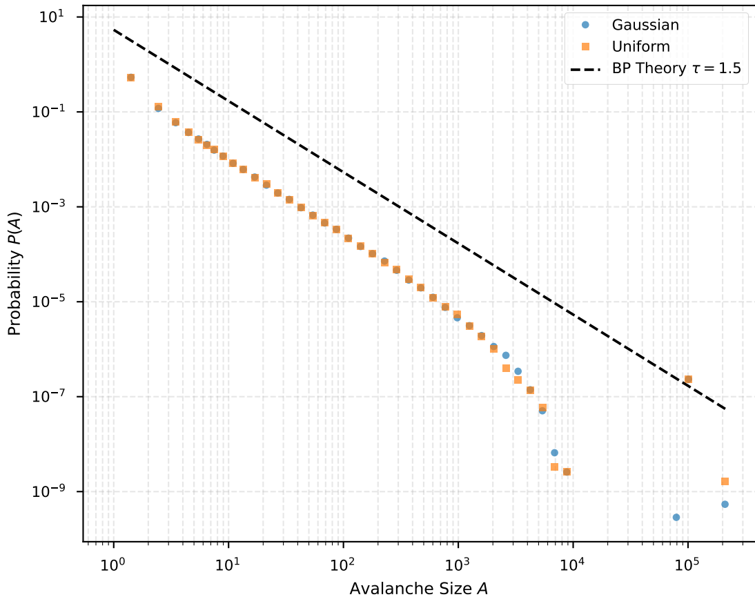
Part 1: Avalanche Size Distribution
