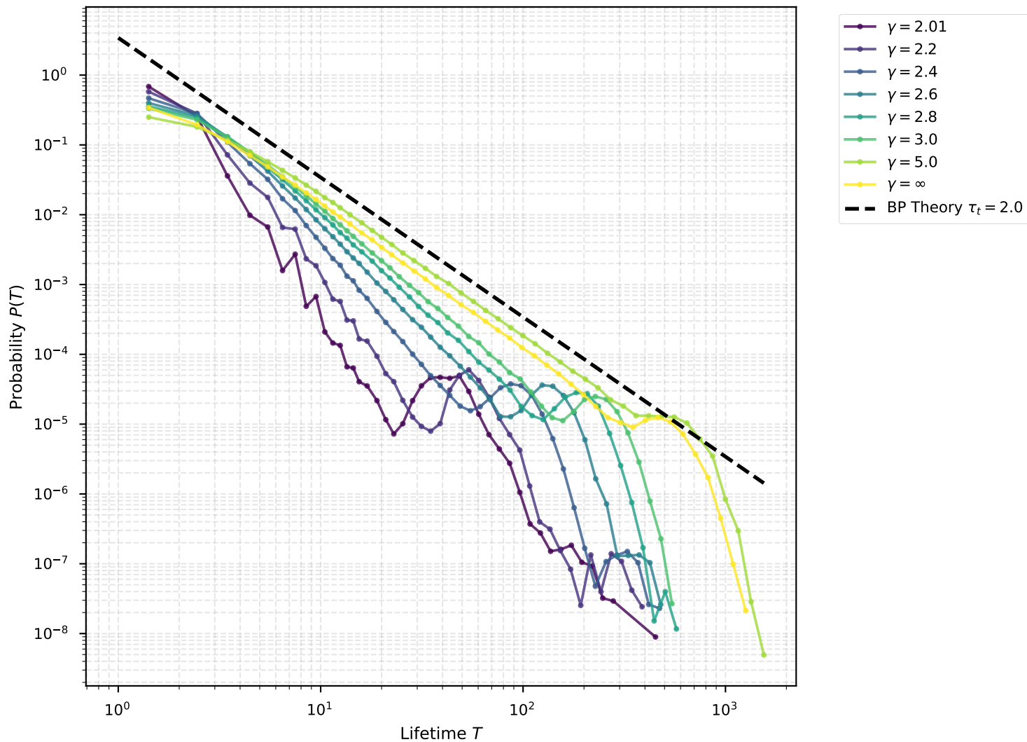
Part 2: Avalanche Lifetime Distribution (Scale-Free)
