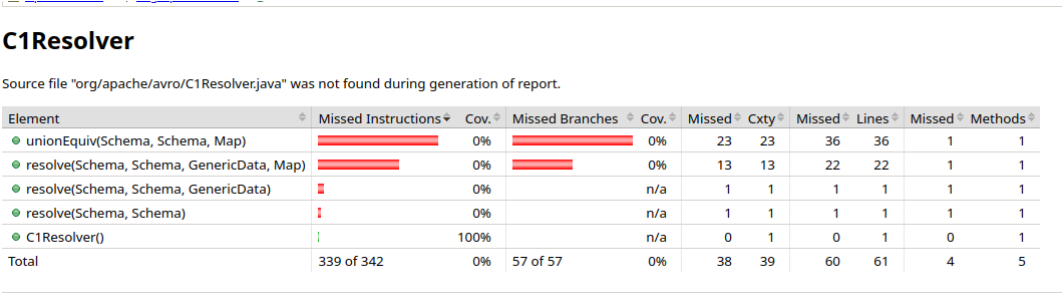
Figure 14: Coverage JaCoCo della suite Randoop su C1Resolver.
