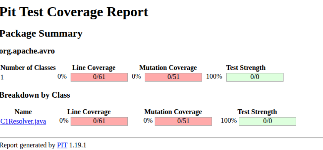
Figure 15: Report PIT della suite Randoop su C1Resolver.
