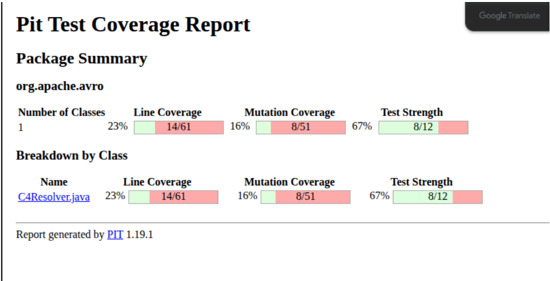
Figure 31: Report PIT della suite LLM ToT su C4Resolver.
