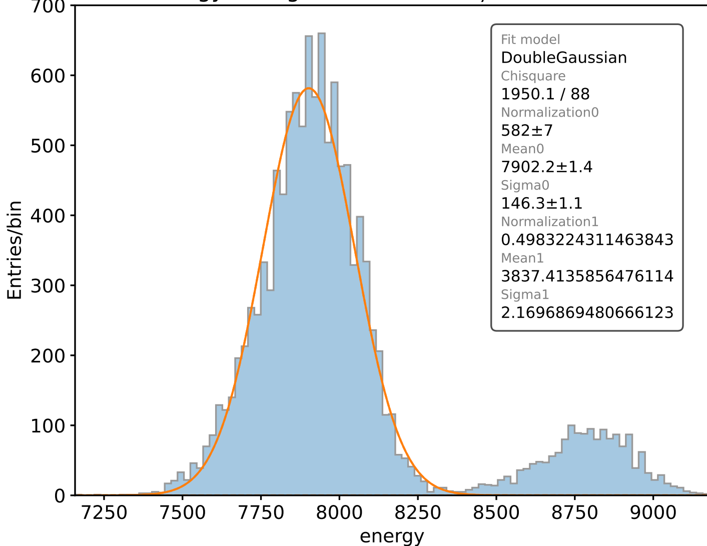
Energy histogram for t = 450 \mu\text{m} , \text{ENC} = 25
