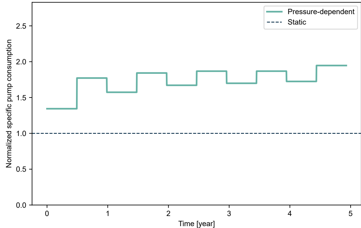
Impact of bhp variations on the pump power consumption
