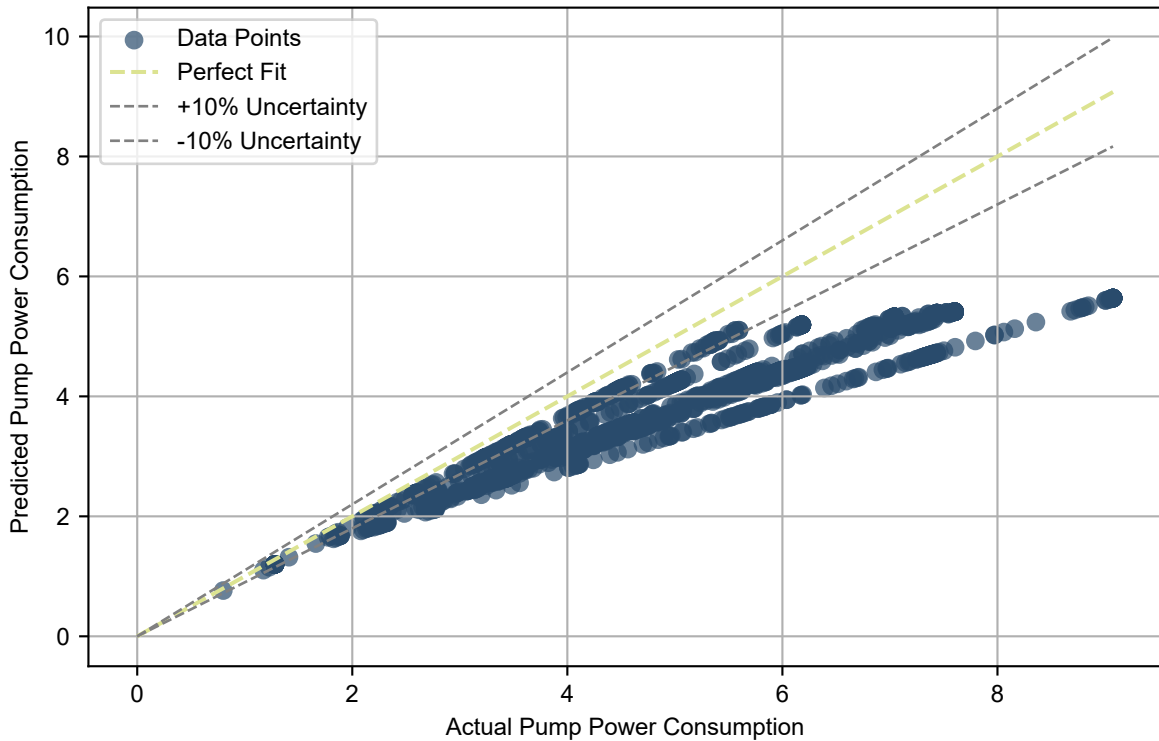
Parity Plot: Predicted vs Actual Pump Power Consumption with \pm 10\% Uncertainty
