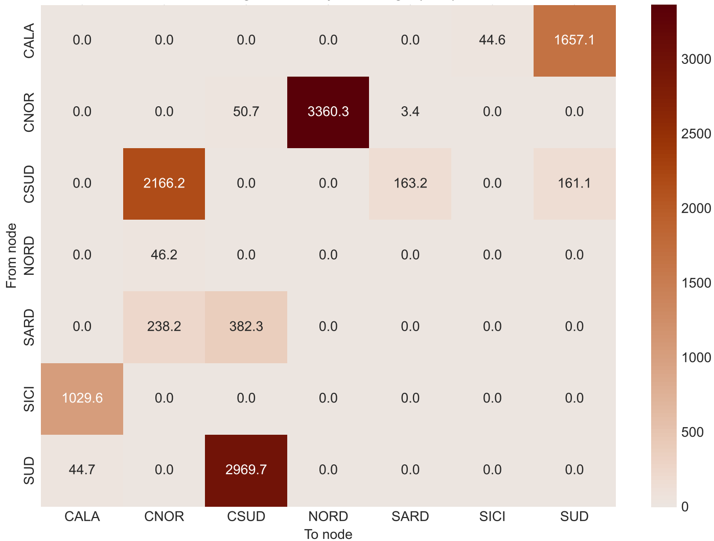
Average Electricity Exchange (MW)
