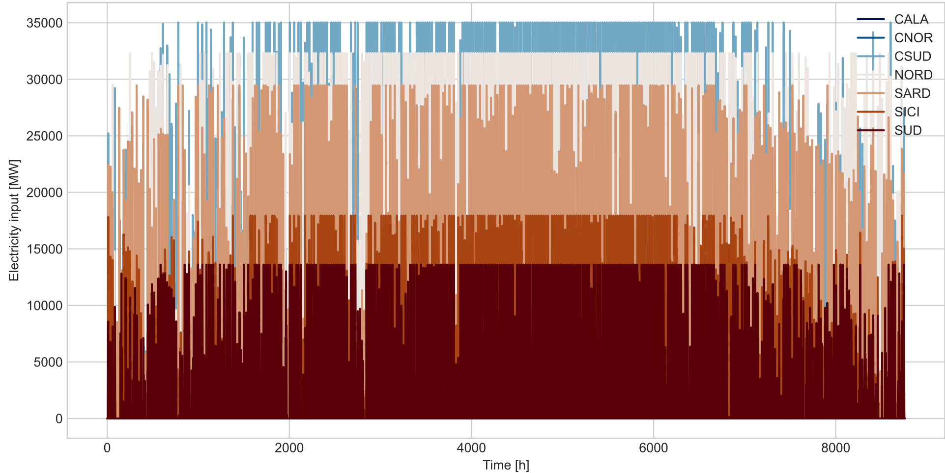
Battery Electricity input Over Time
