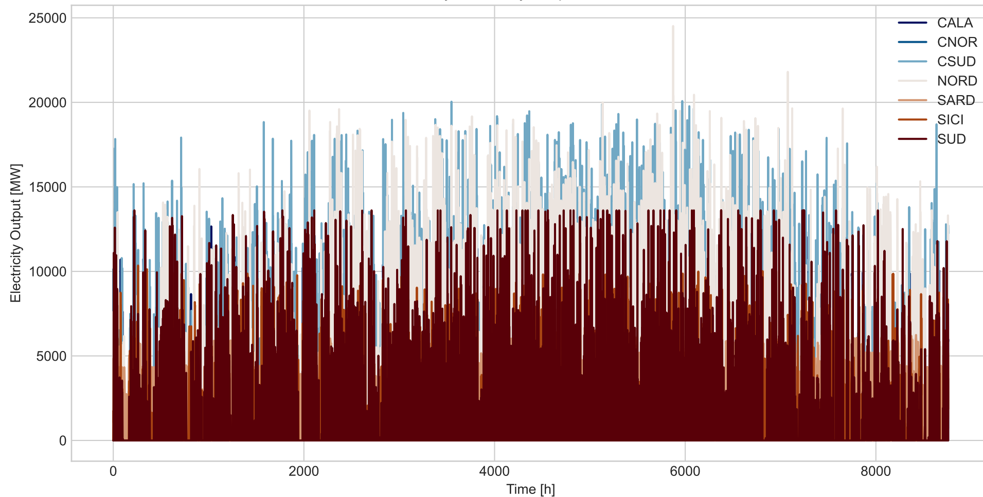
Battery Electricity Output Over Time
