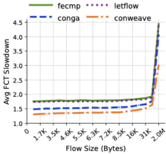
Figure 2: Average FCT slowdown vs flow size (Lossless RDMA, 50 % load). Corresponds to Figure 12(a) in the paper.
