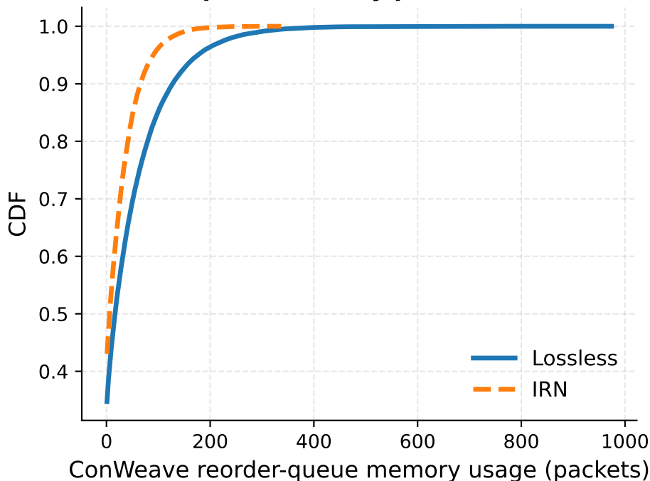
Reorder-queue memory per ToR (50% load)
