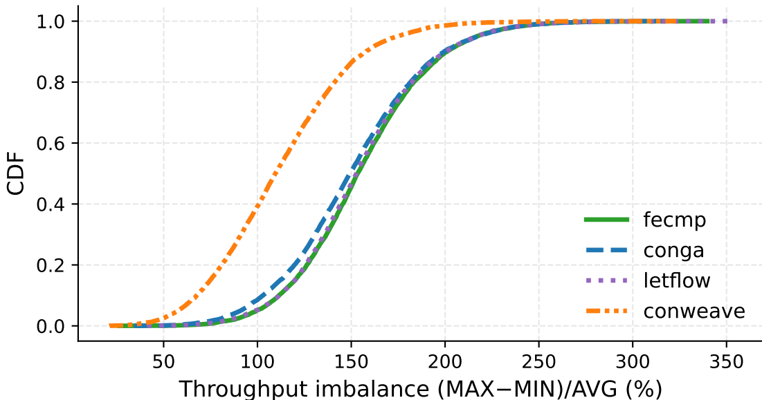
Uplink throughput imbalance (IRN, 50% load)
