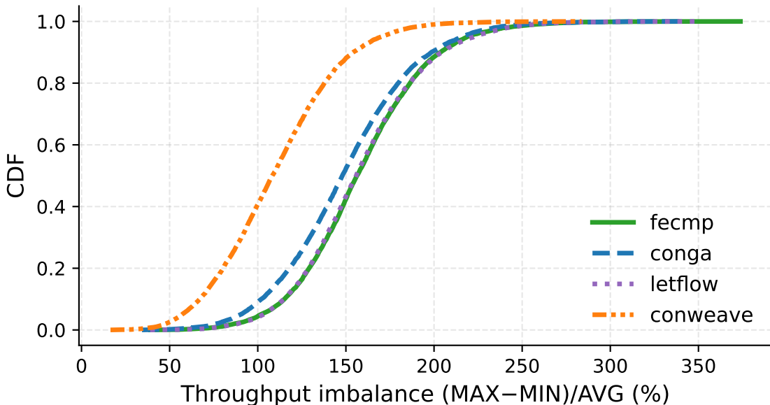
Uplink throughput imbalance (Lossless, 50% load)
