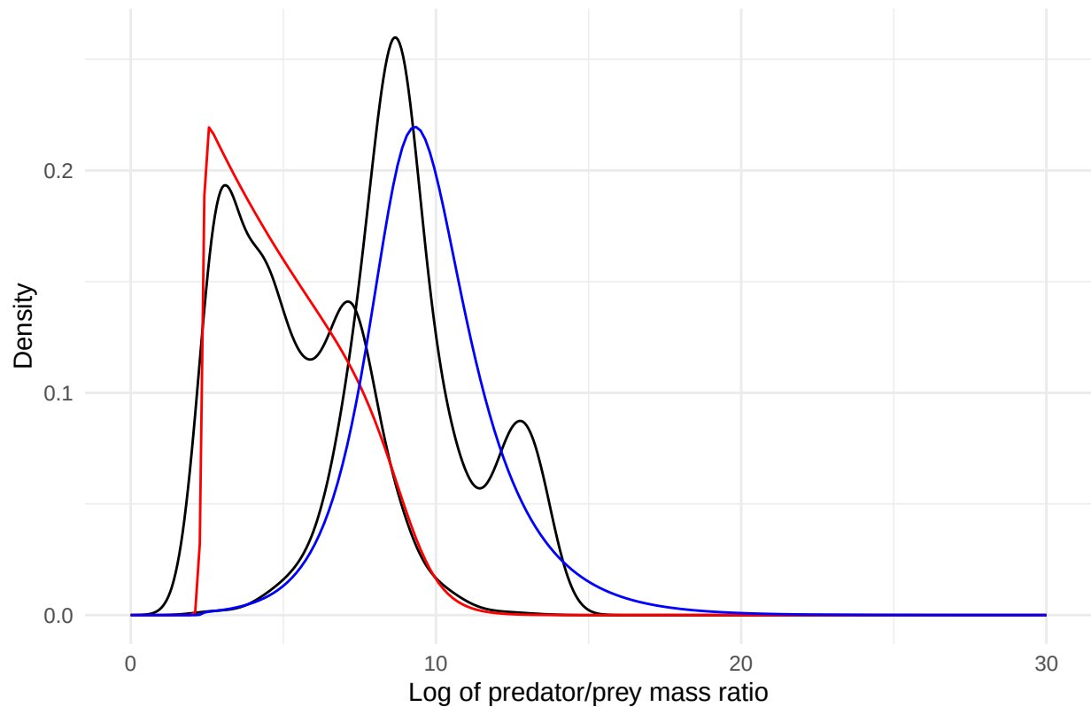
Blue Whiting – Fitted to Biomass, shift to number
