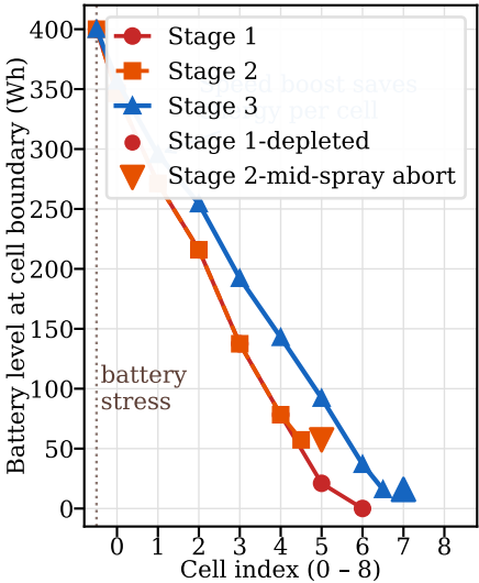
Battery per cell — speed boost (Sc C) preserves more battery than full-speed scenarios (Sc A / B) after motor failure
