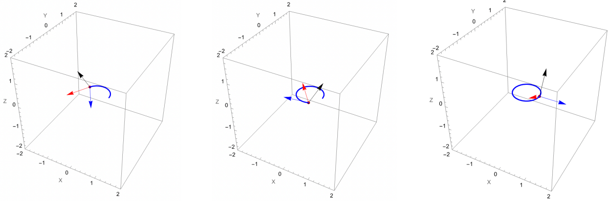
Figure 3: Triad representations at different positions s along the rod. The red arrow represents \mathbf{D}^1 , the blue arrow represents \mathbf{D}^2 , and the black arrow represents \mathbf{D}^3 . Notice that \mathbf{D}^3 does not point in the direction tangent to the curve as per the original Kirchhoff rod constraints. Instead, the IB method imposes the energy penalty function that tends to maintain these constraints.
