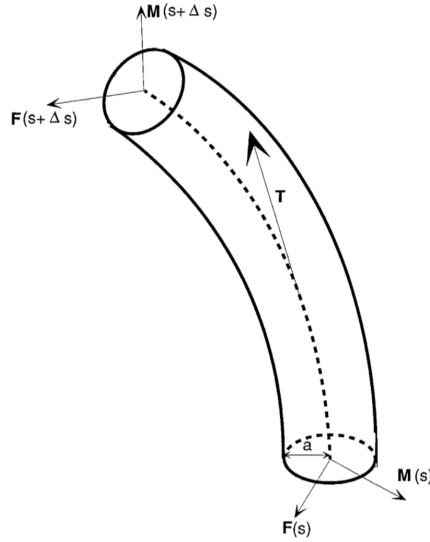
Figure 2: A depiction of a Kirchhoff Rod [3]. Here, T is constrained to be tangent to the curve. F and M give the force and moment from the rod, respectively.
