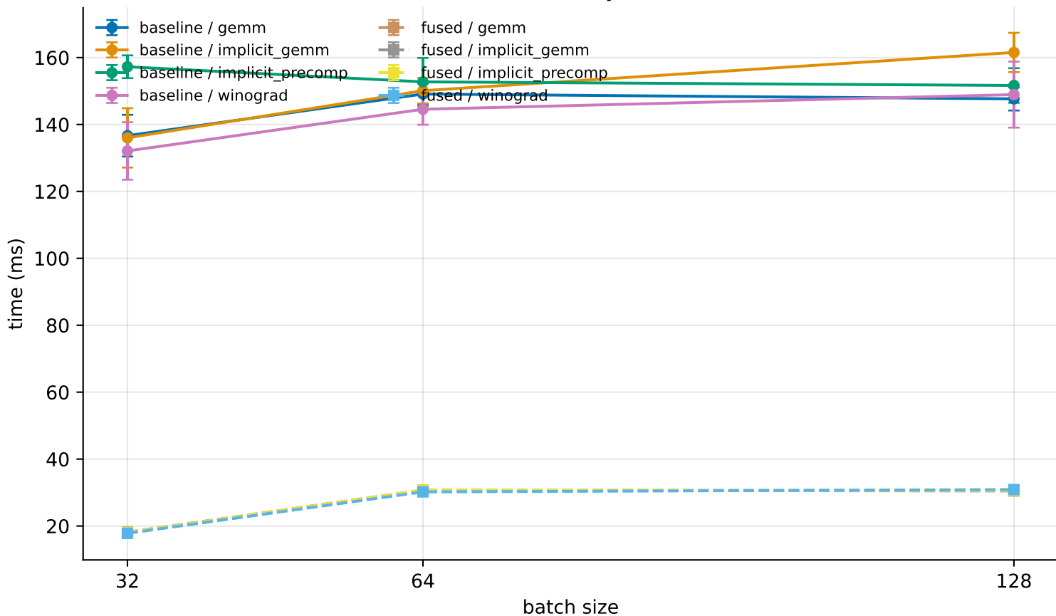
LeNet forward latency vs batch size
