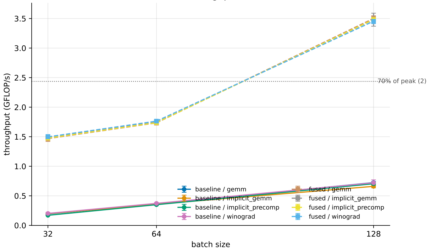
LeNet forward throughput vs batch size
