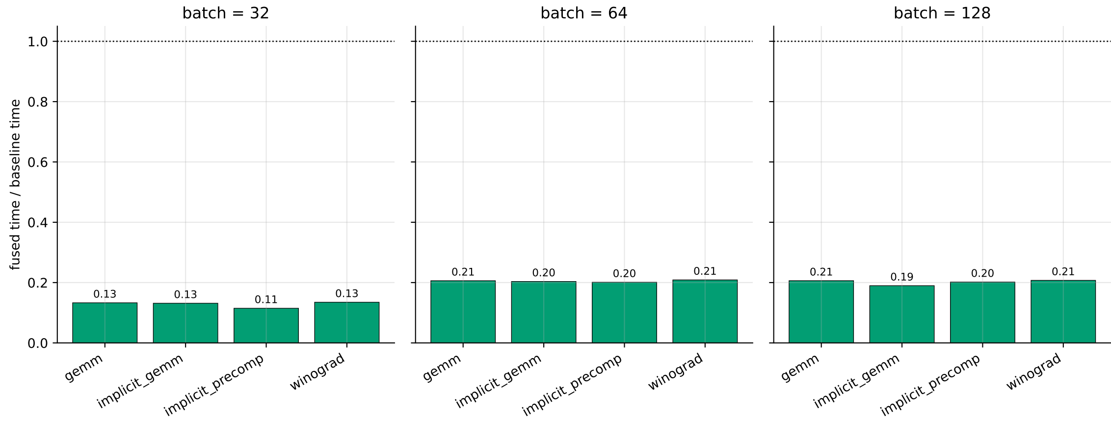
Fusion speedup (values < 1.0 mean fused is faster)
