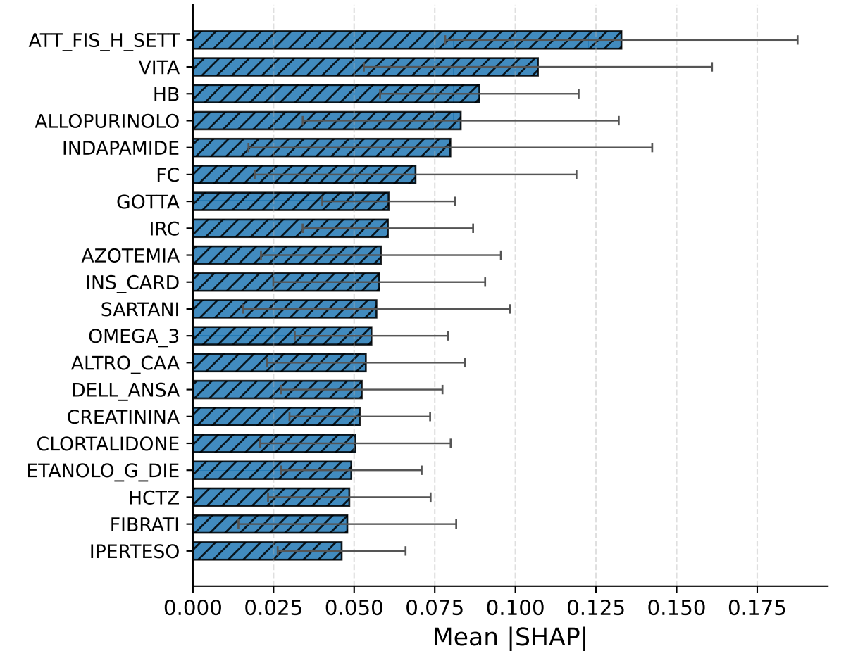
DeepSurv MLP (Baseline)
